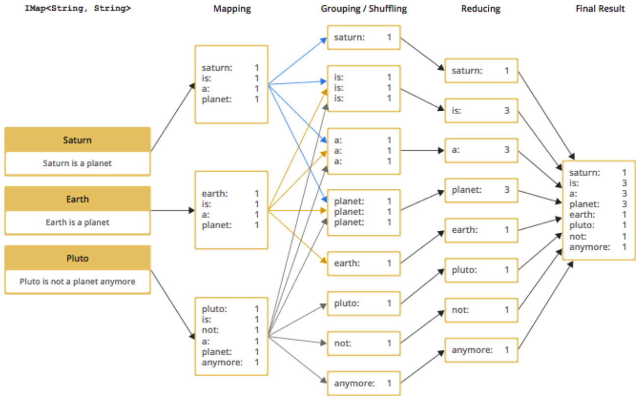
Figure 10.1: MapReduce Workflow
