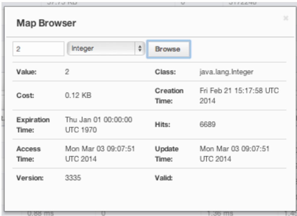
Figure 18.18: Map Browser
