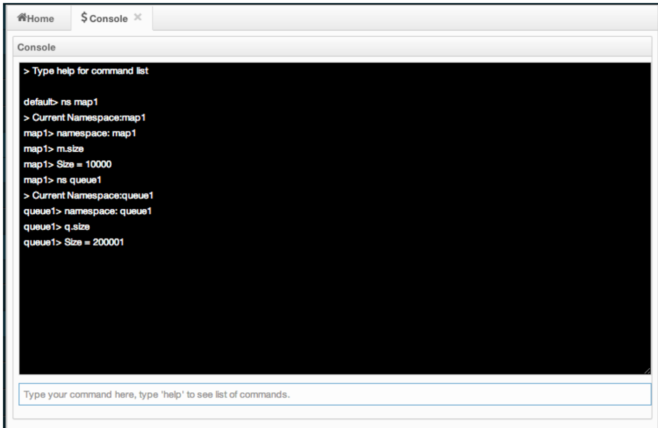
Figure 18.38: Console
