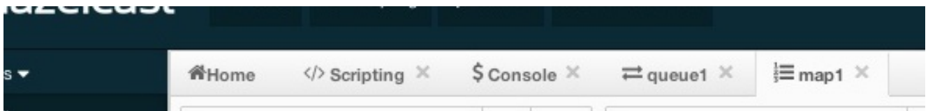
Figure 18.10: Tabbed View
