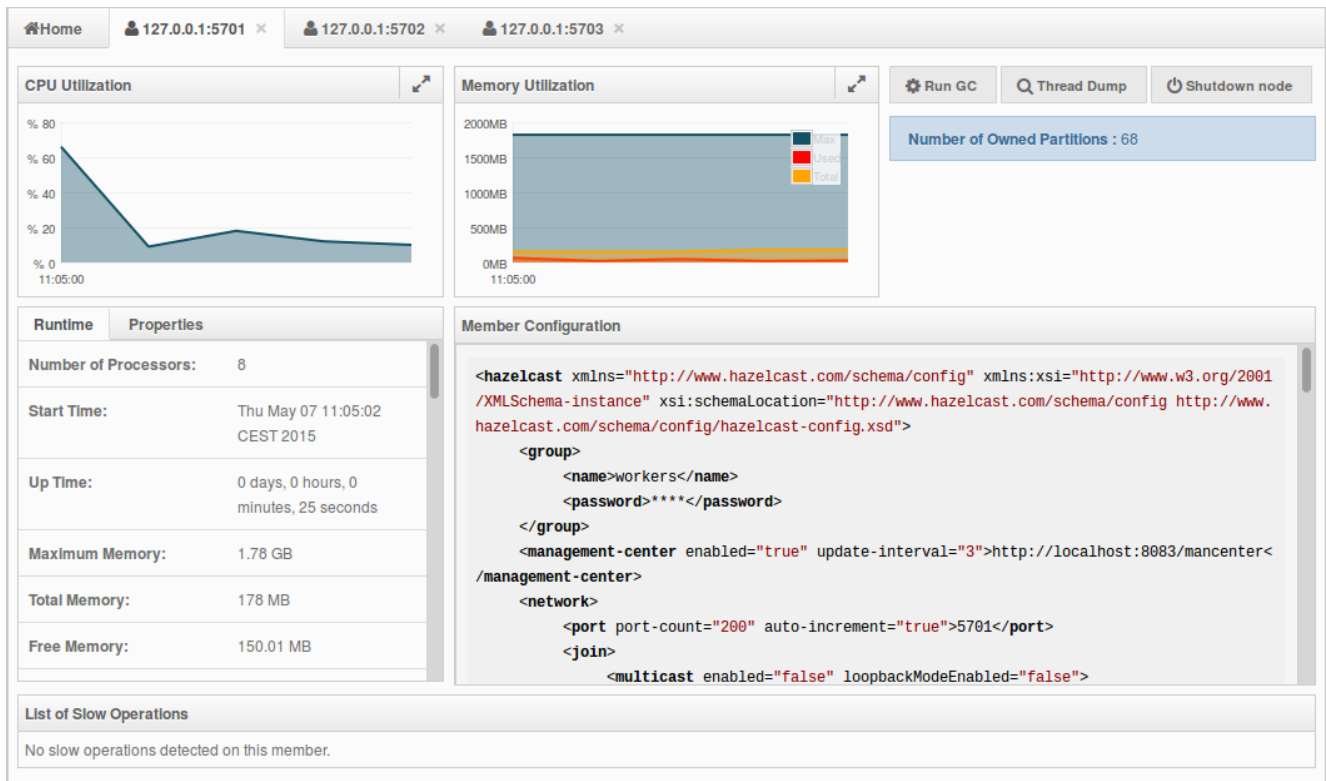
Figure 18.34: Monitoring Members
