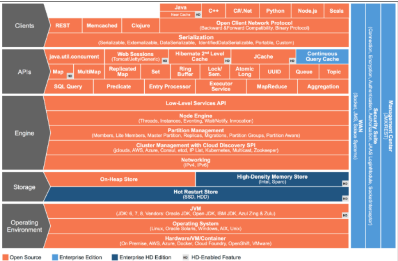
Figure 1.1: Hazelcast Architecture
