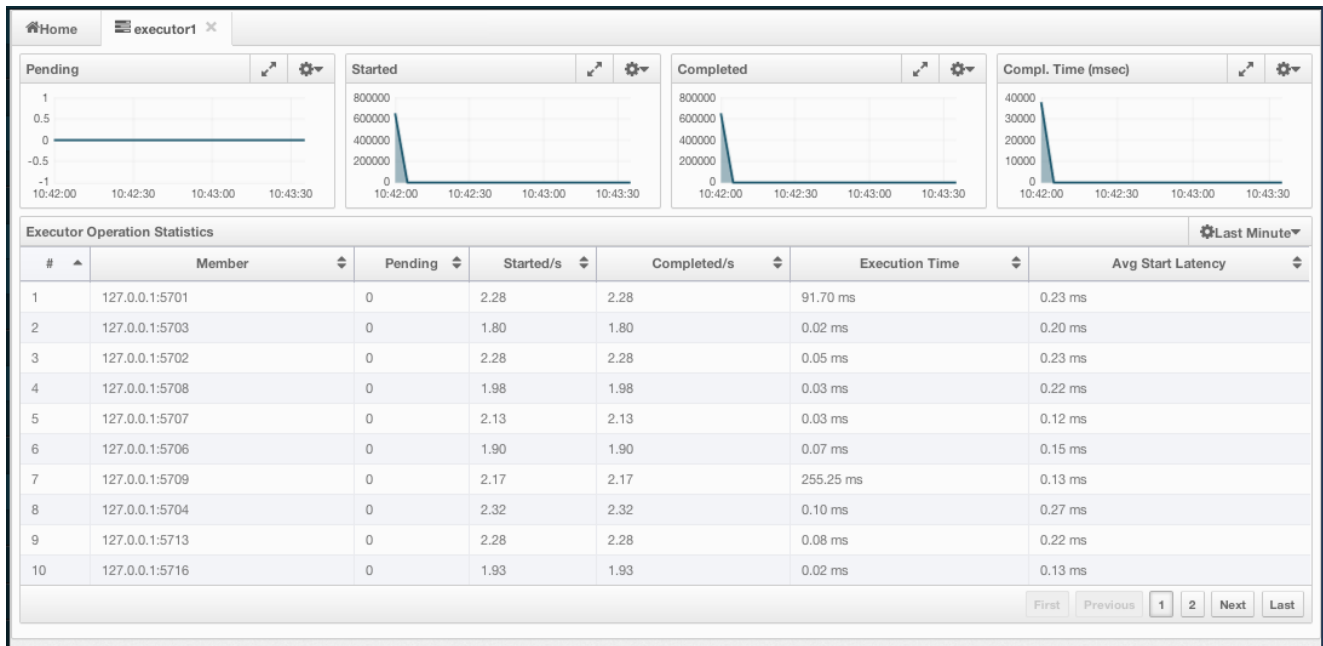
Figure 18.29: Monitoring Executors
