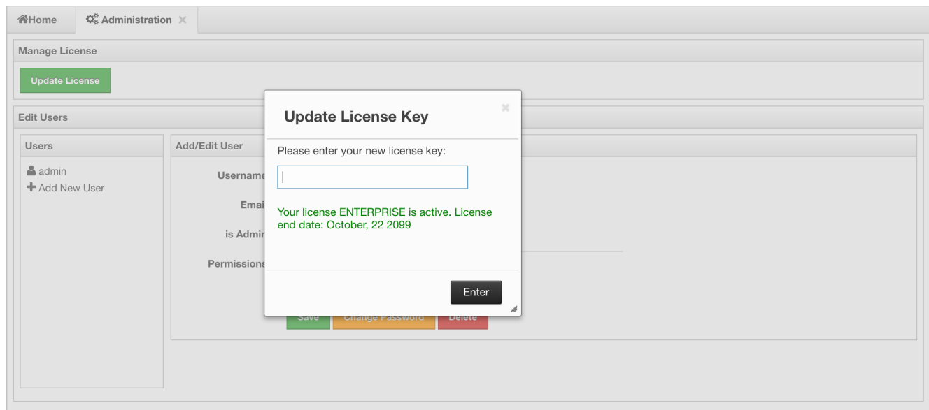
Figure 18.45: License
