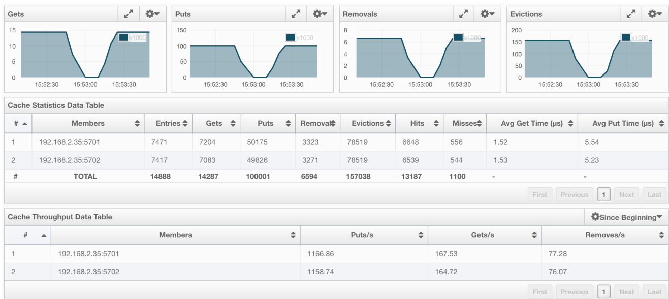
Figure 18.16: Monitoring Caches
