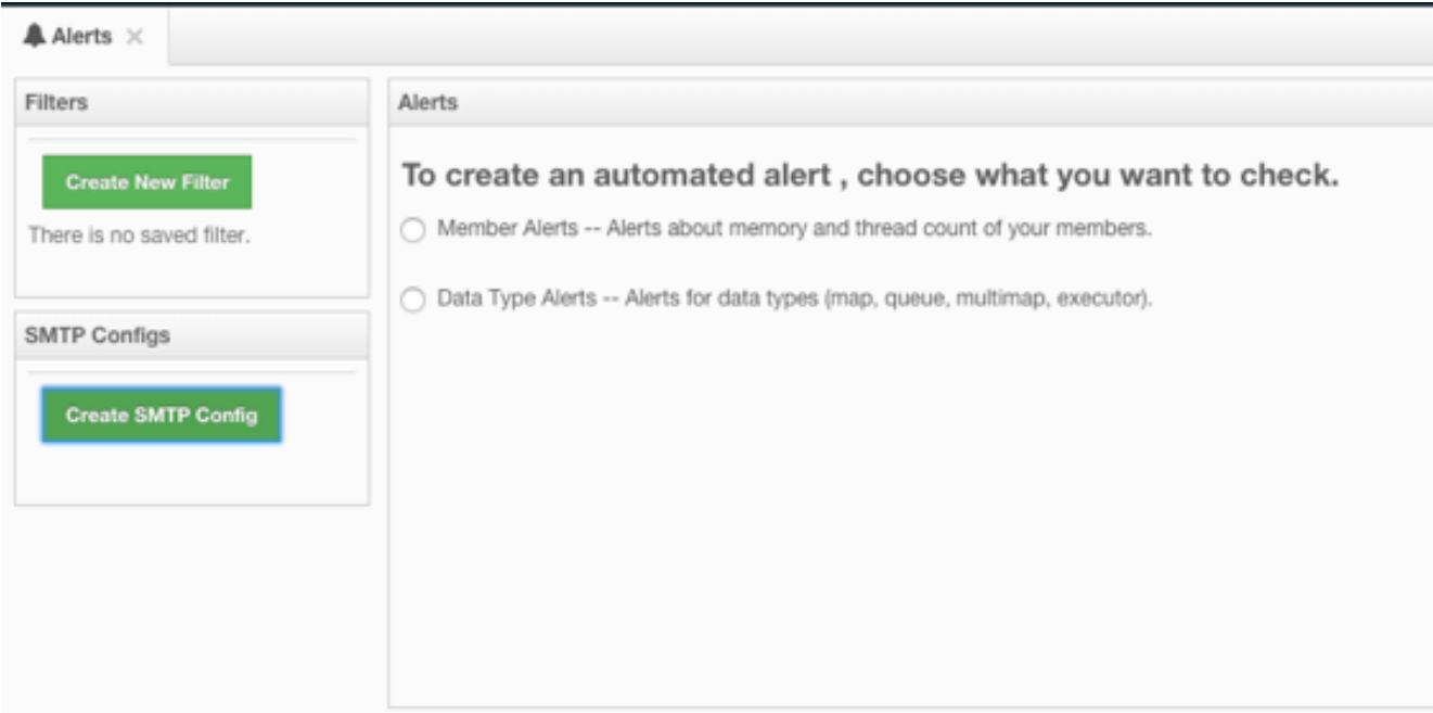
Figure 18.39: Creating Alerts
