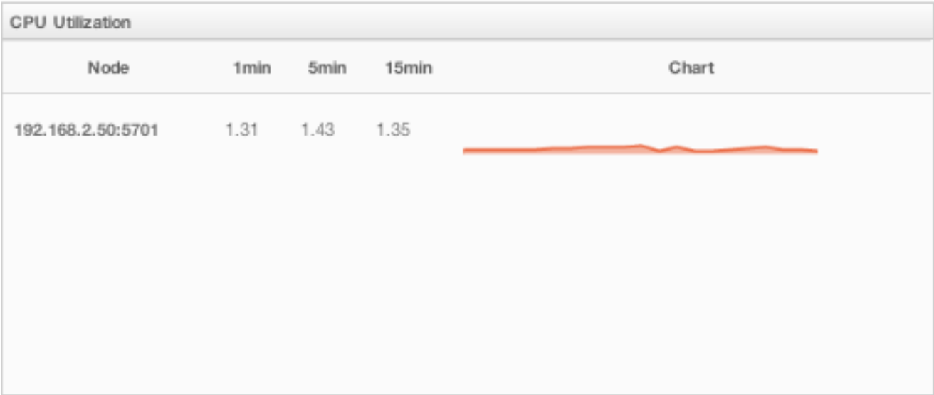
Figure 18.11: CPU Utilization
