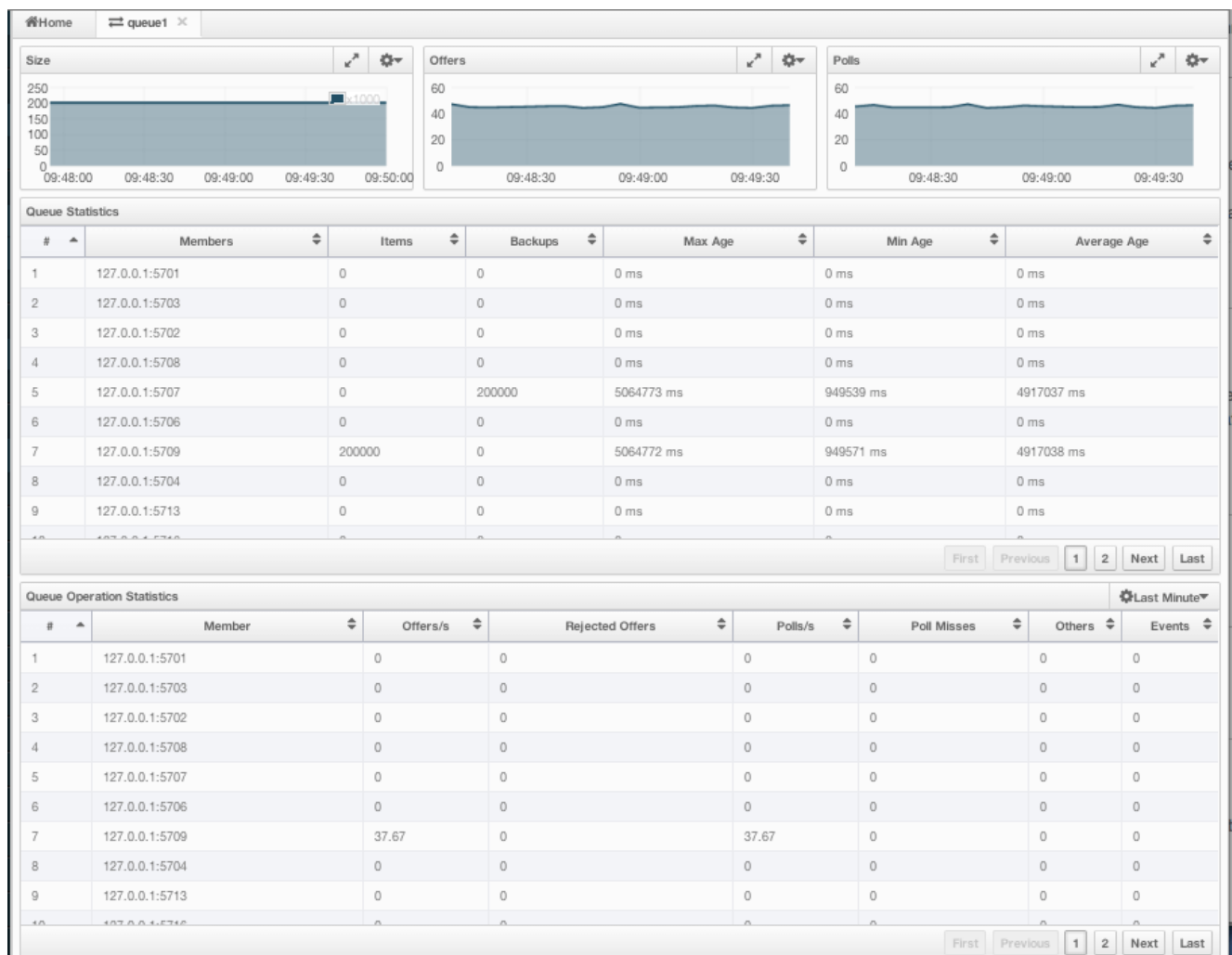
Figure 18.24: Monitoring Queues
