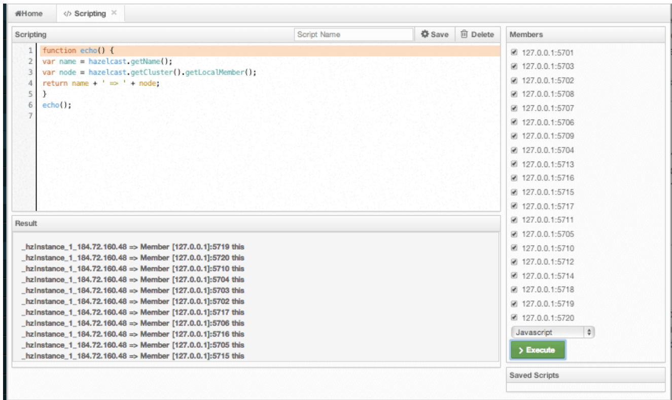
Figure 19.39: Scripting
