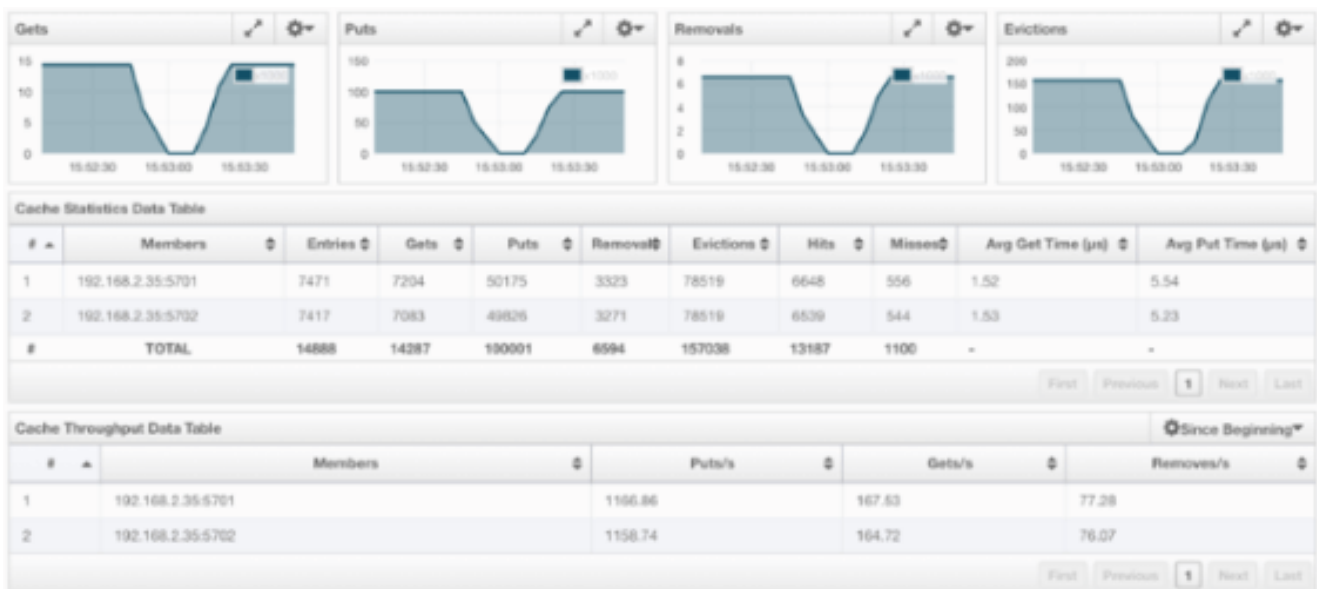
Figure 19.18: Monitoring Caches
