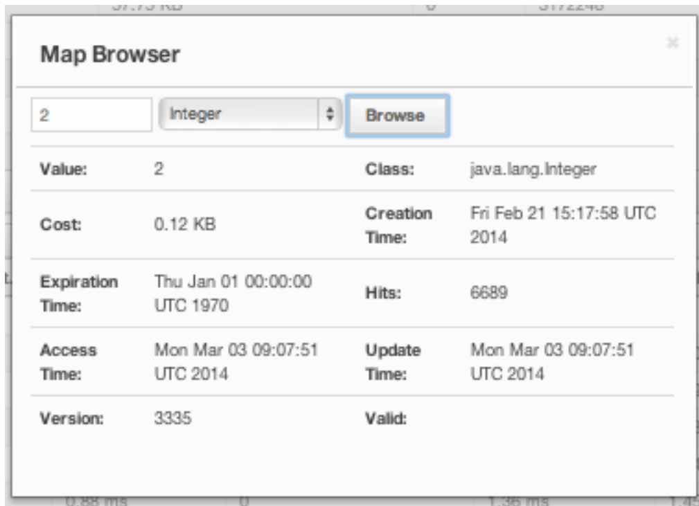
Figure 19.20: Map Browser
