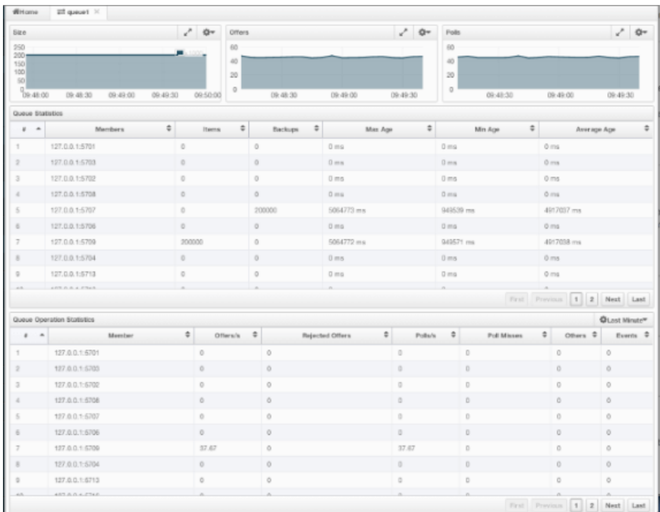
Figure 19.27: Monitoring Queues
