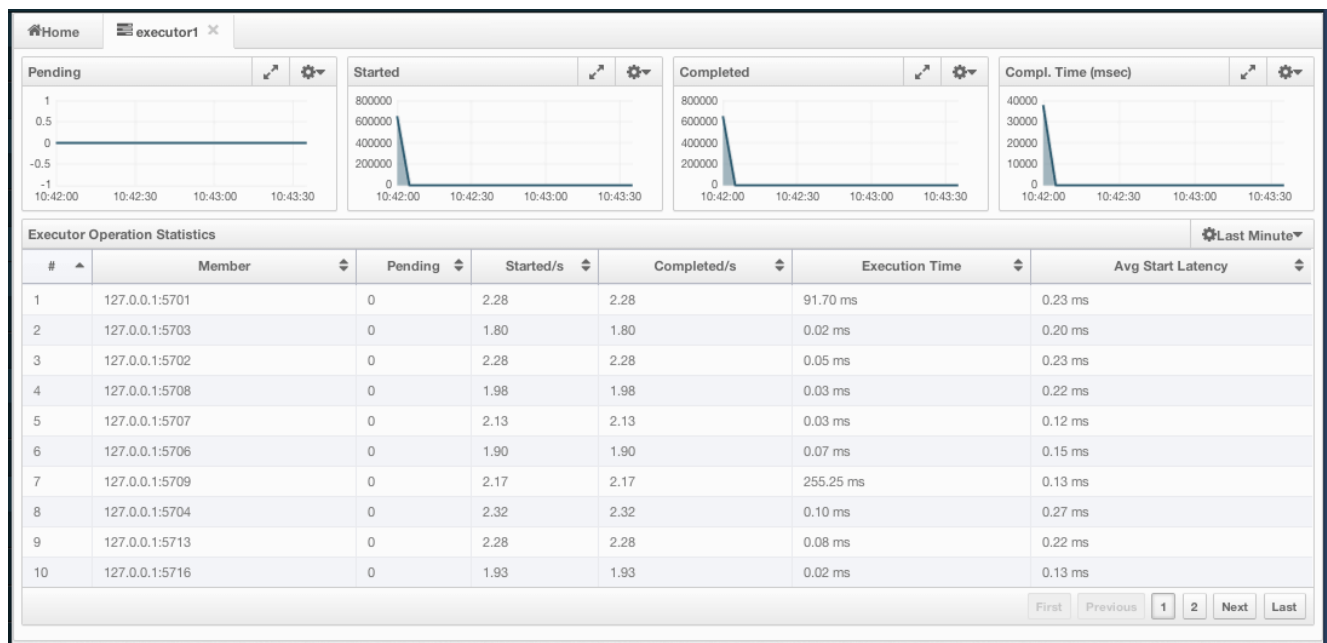
Figure 19.31: Monitoring Executors
