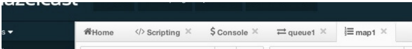
Figure 19.12: Tabbed View
