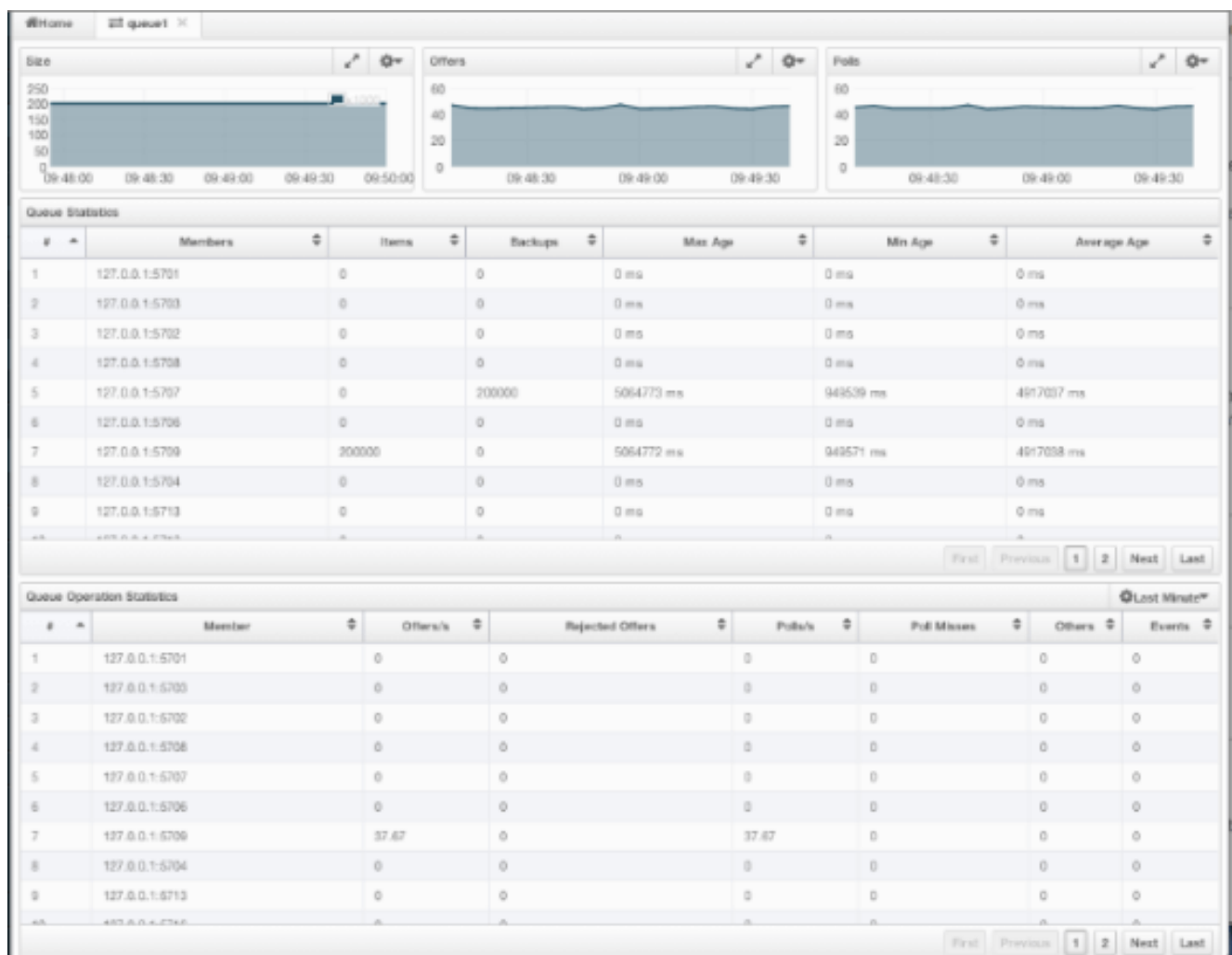
Figure 19.27: Monitoring Queues
