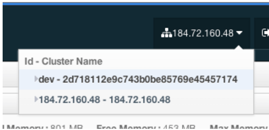
Figure 19.10: Changing Cluster
