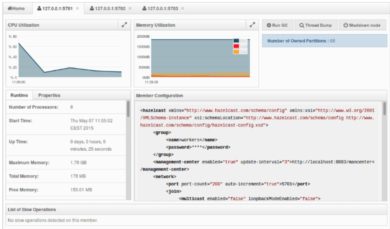
Figure 19.36: Monitoring Members
