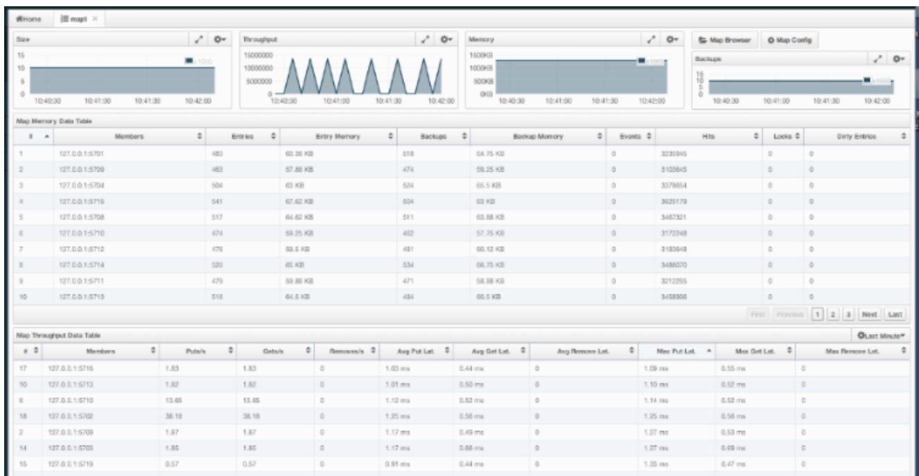
Figure 19.19: Monitoring Maps
