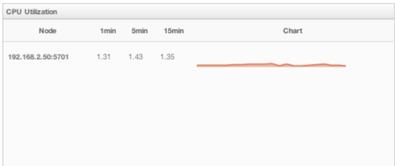
Figure 19.13: CPU Utilization
