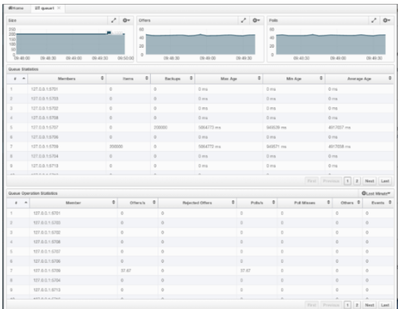
Figure 19.27: Monitoring Queues
