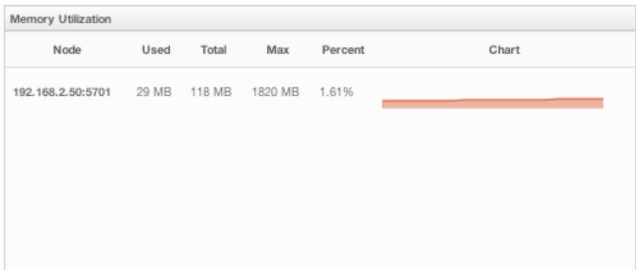
Figure 19.14: Memory Utilization
