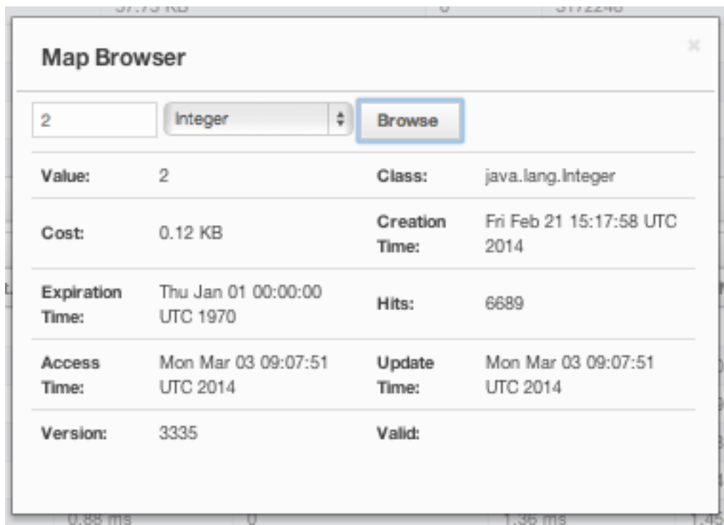
Figure 19.20: Map Browser
