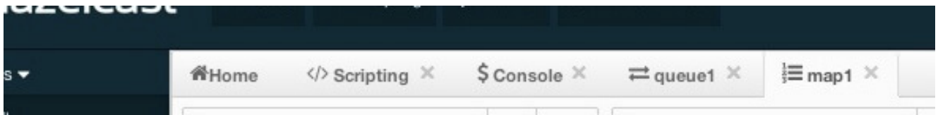
Figure 19.12: Tabbed View
