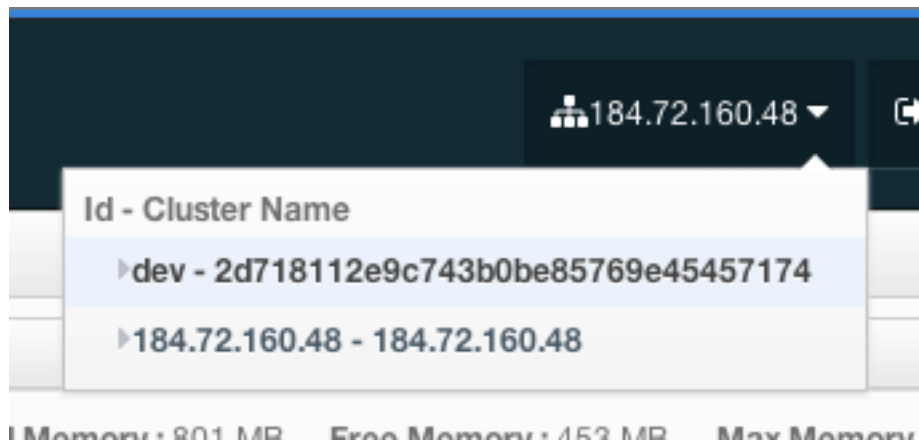
Figure 19.10: Changing Cluster
