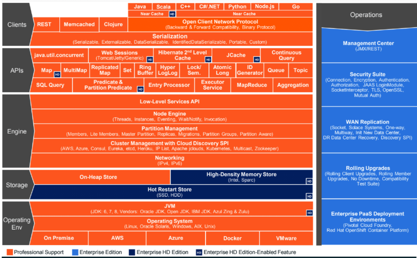
Figure 1.1: Hazelcast Architecture
