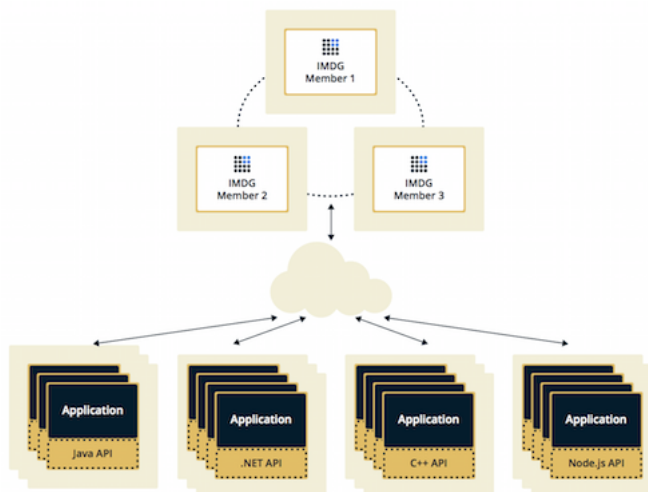
Figure 4.2: Client/Server Deployment
