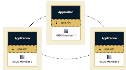
Figure 4.1: Embedded Deployment
